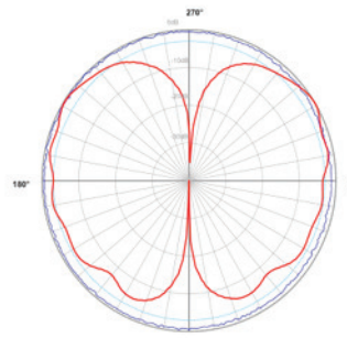
1710-2155 MHz Upper 2 dBi Gain
