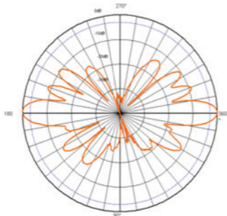
1710-2155 MHz Lower 9 dBi Gain
