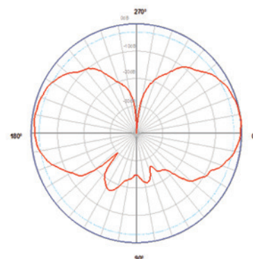
698-896 MHz Upper 2 dBi Gain
