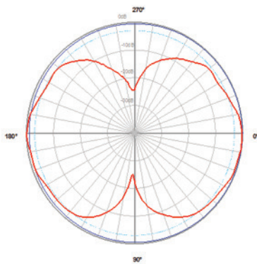
698-896 MHz Lower 2 dBi Gain
