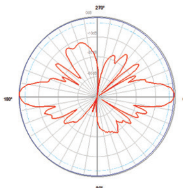
1710-2155 MHz Middle 9 dBi Gain
