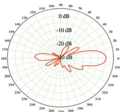
1695-2180 MHz Elevation Pattern
