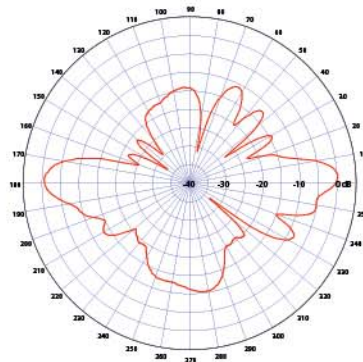
Elevation Pattern
